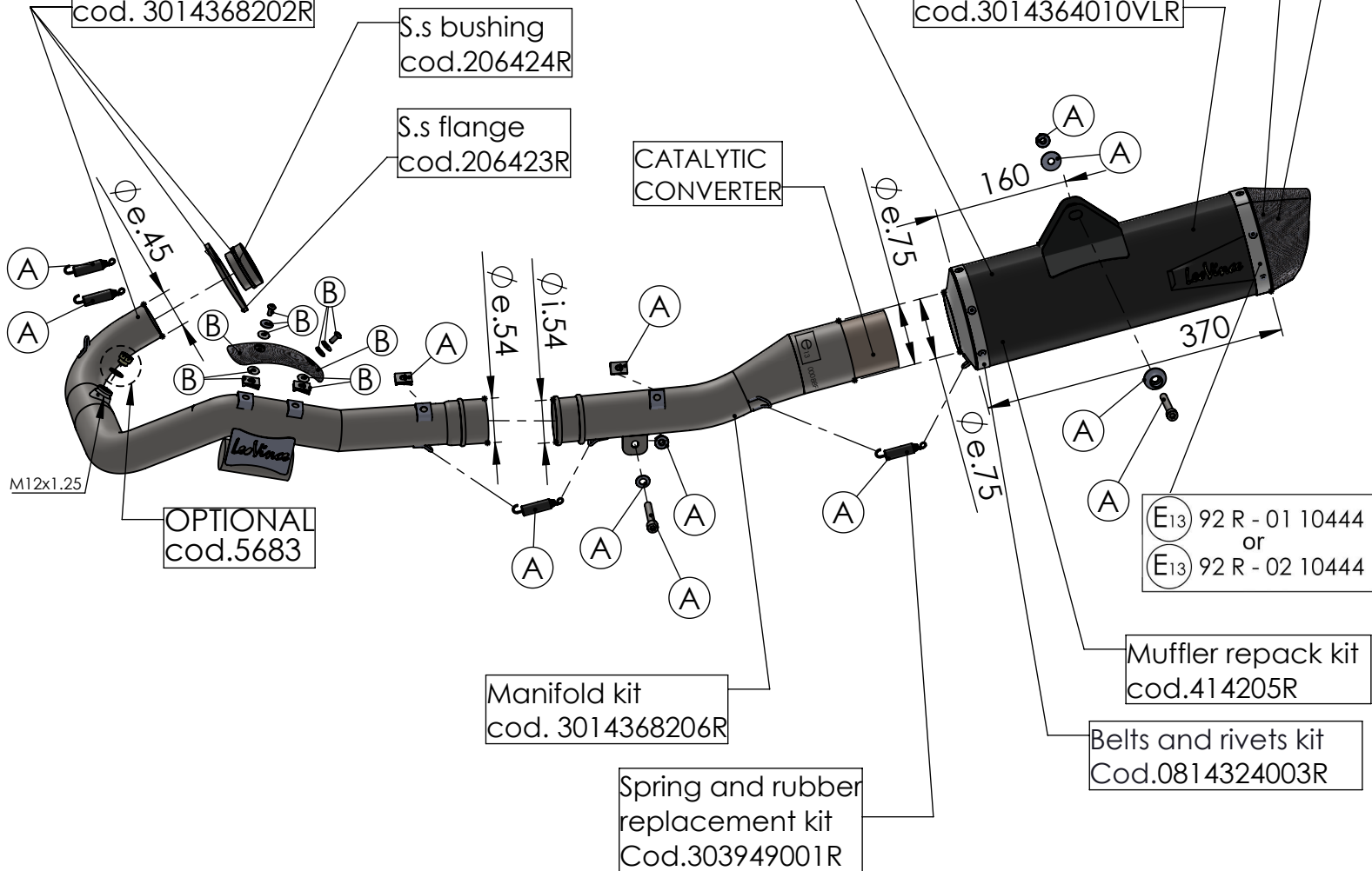
Outer sleeve replacement kit cod.3014364010VLR
